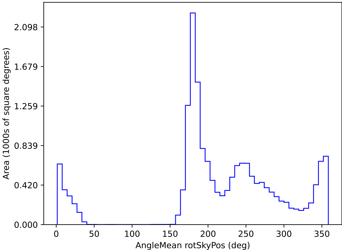
ddf_loaded_fl15_v3.4_10yrs WFD i band: AngleMean rotSkyPos
