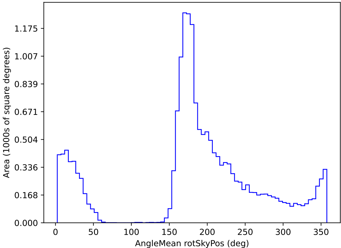
ddf_loaded_fl15_v3.4_10yrs WFD g band: AngleMean rotSkyPos
