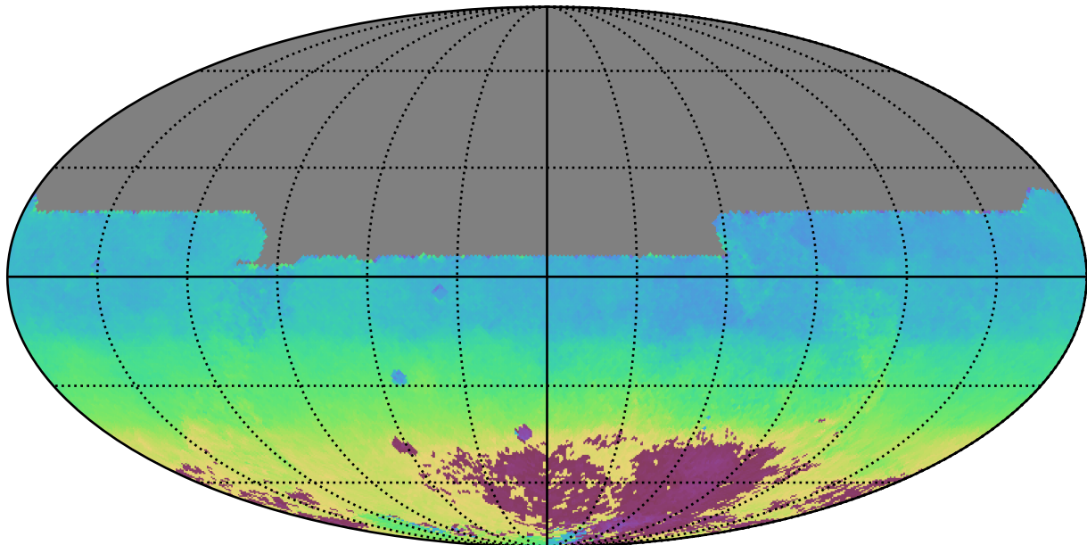
ddf_loaded_fl15_v3.4_10yrs All sky y band: AngleMean rotSkyPos
