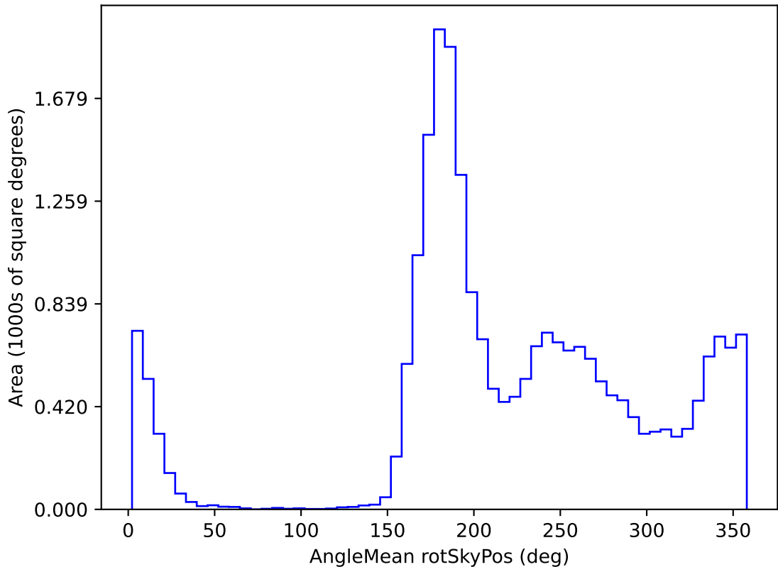
ddf_loaded_fl15_v3.4_10yrs All sky y band: AngleMean rotSkyPos
