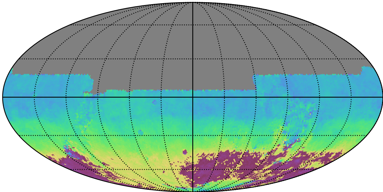
ddf_loaded_fl15_v3.4_10yrs All sky u band: AngleMean rotSkyPos
