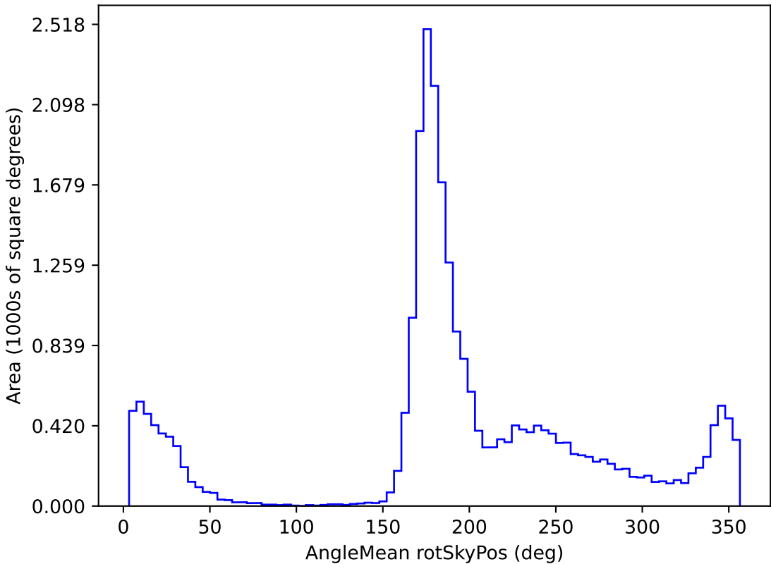
ddf_loaded_fl15_v3.4_10yrs All sky r band: AngleMean rotSkyPos
