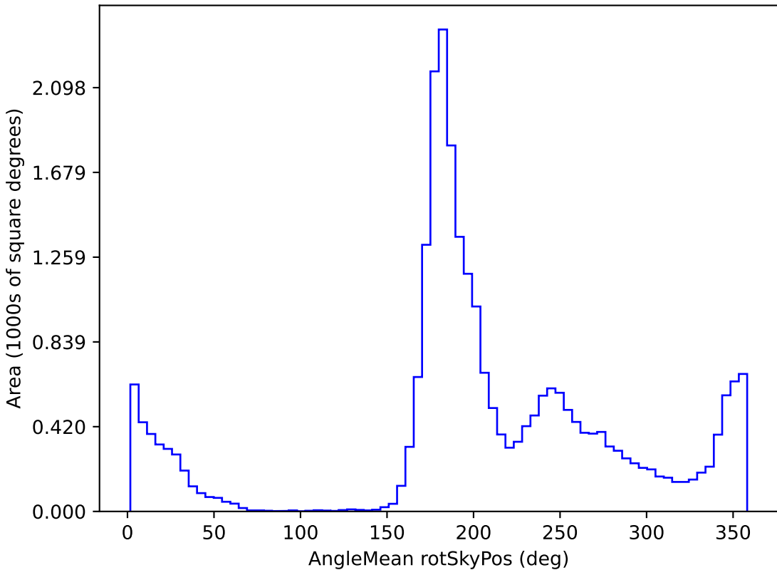
ddf_loaded_fl15_v3.4_10yrs All sky i band: AngleMean rotSkyPos
