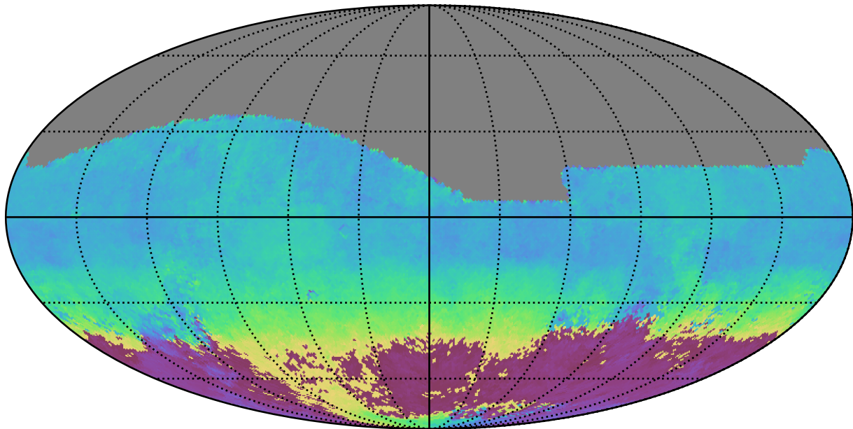
ddf_loaded_fl15_v3.4_10yrs All sky g band: AngleMean rotSkyPos
