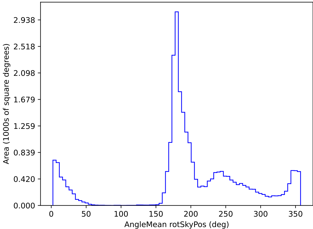
ddf_loaded_fl15_v3.4_10yrs All sky all bands: AngleMean rotSkyPos
