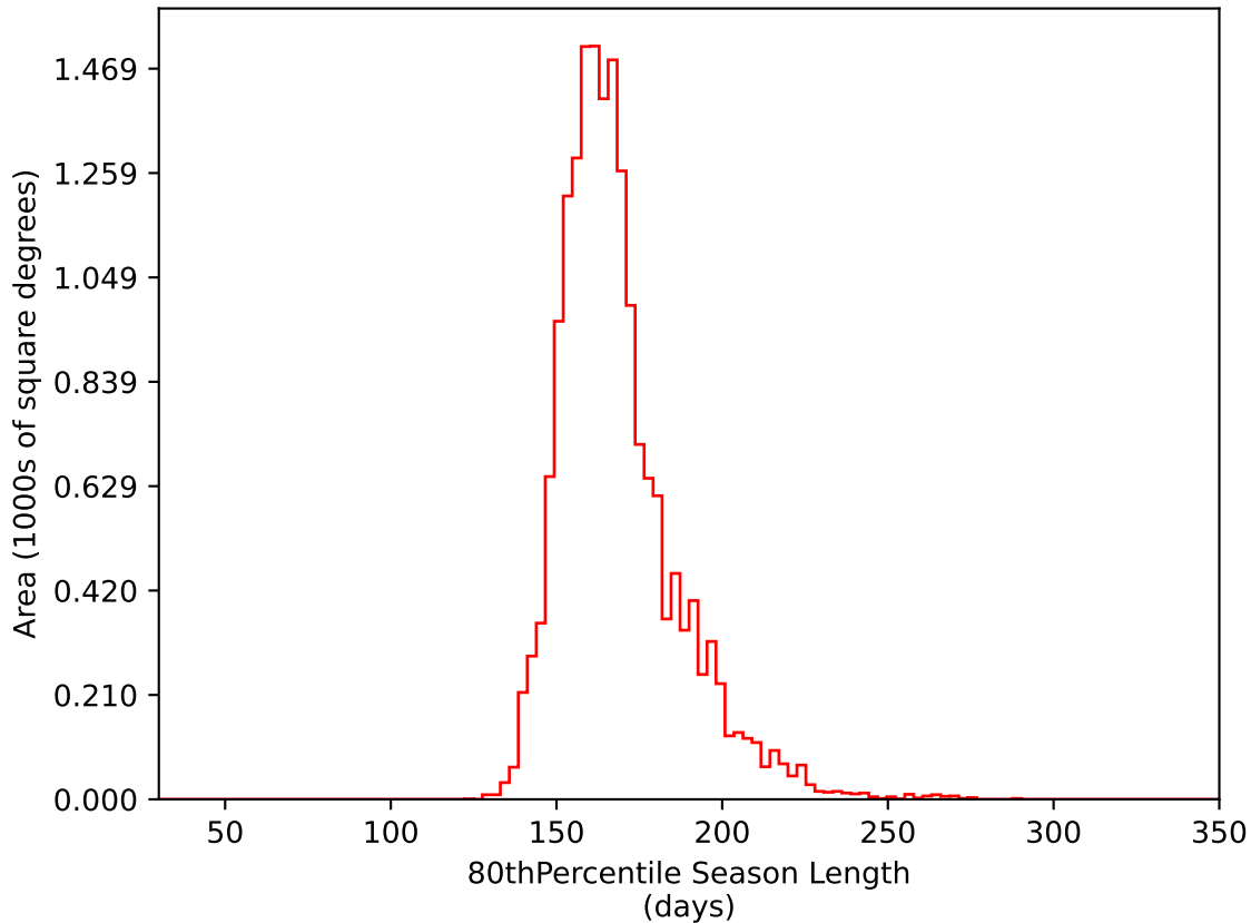
ddf_loaded_fl15_v3.4_10yrs WFD i band: 80thPercentile Season Length
