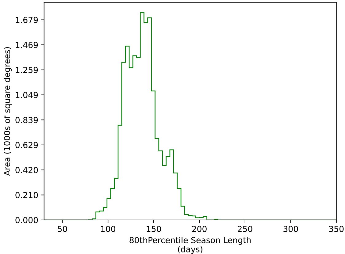
ddf_loaded_fl15_v3.4_10yrs WFD g band: 80thPercentile Season Length
