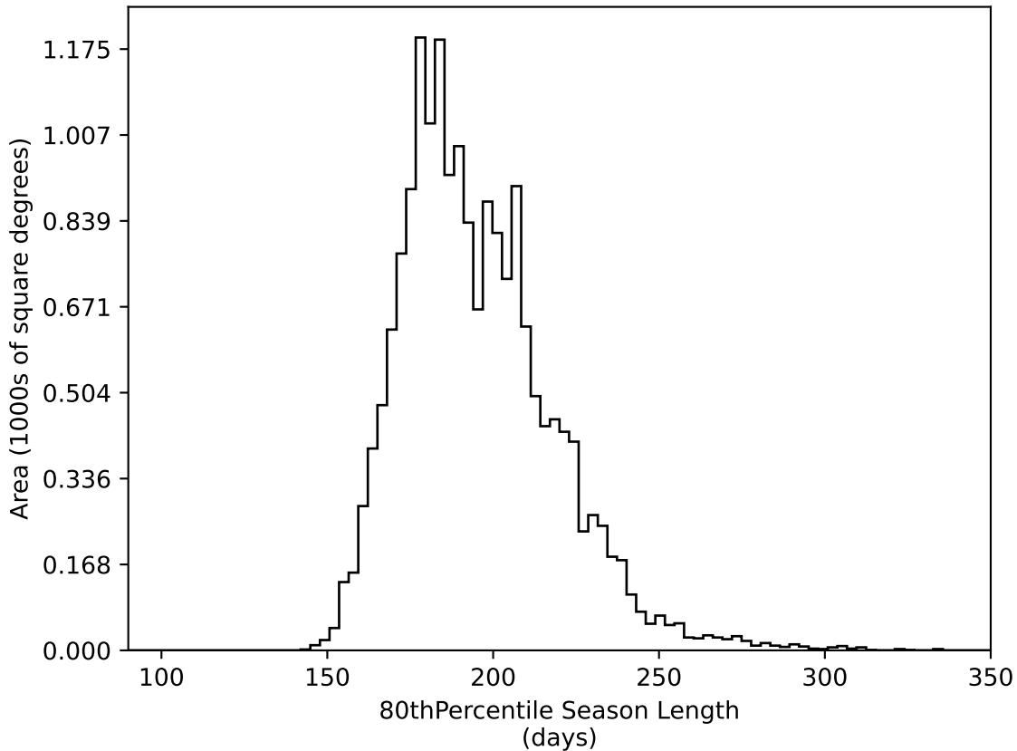
ddf_loaded_fl15_v3.4_10yrs WFD all bands: 80thPercentile Season Length
