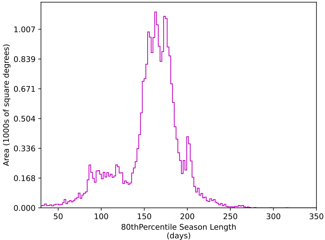
ddf_loaded_fl15_v3.4_10yrs All sky z band: 80thPercentile Season Length
