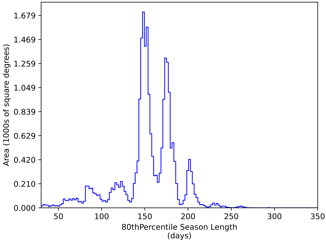
ddf_loaded_fl15_v3.4_10yrs All sky y band: 80thPercentile Season Length
