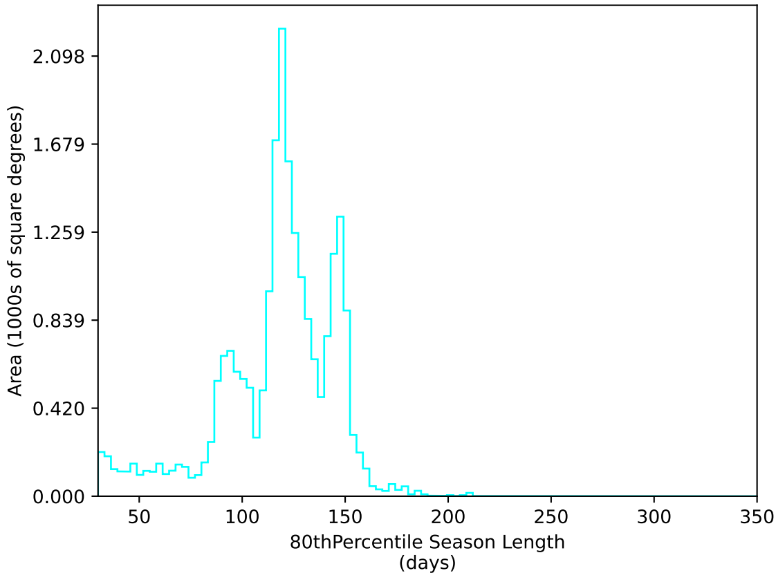
ddf_loaded_fl15_v3.4_10yrs All sky u band: 80thPercentile Season Length
