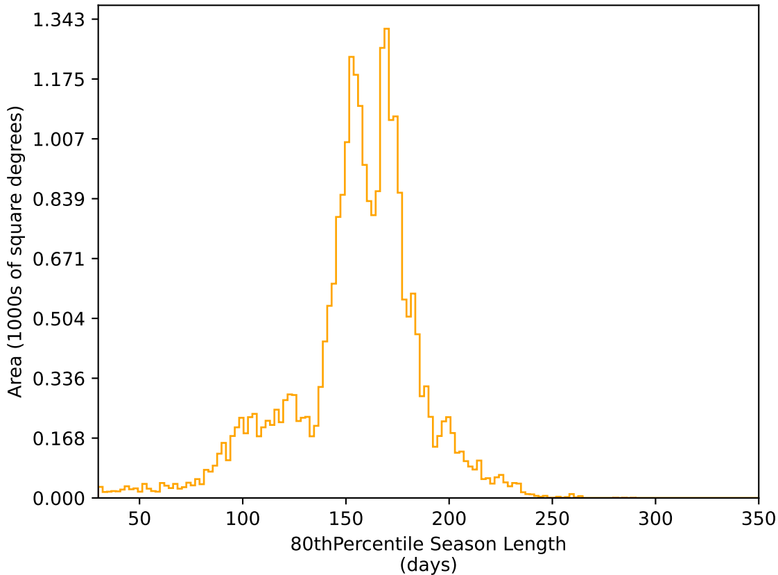
ddf_loaded_fl15_v3.4_10yrs All sky r band: 80thPercentile Season Length
