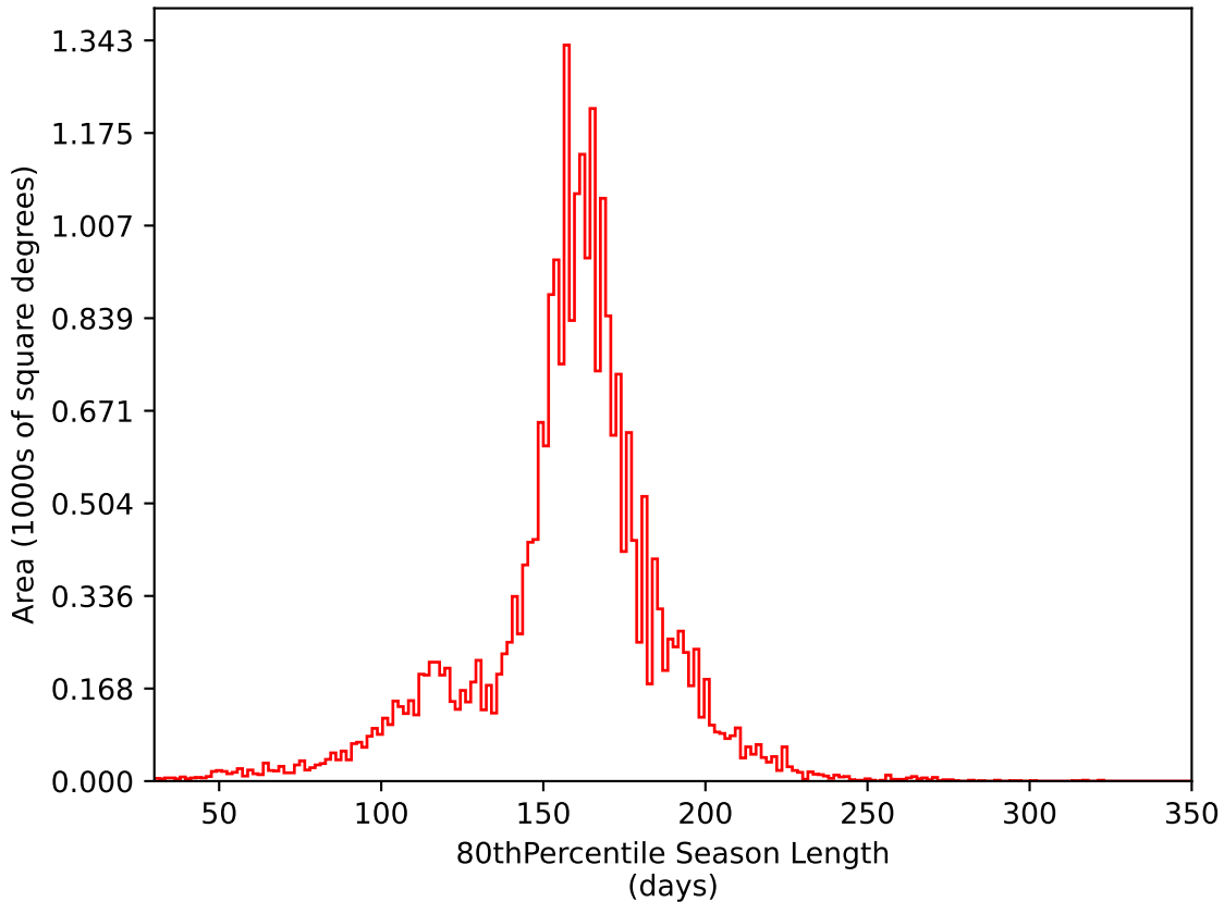
ddf_loaded_fl15_v3.4_10yrs All sky i band: 80thPercentile Season Length
