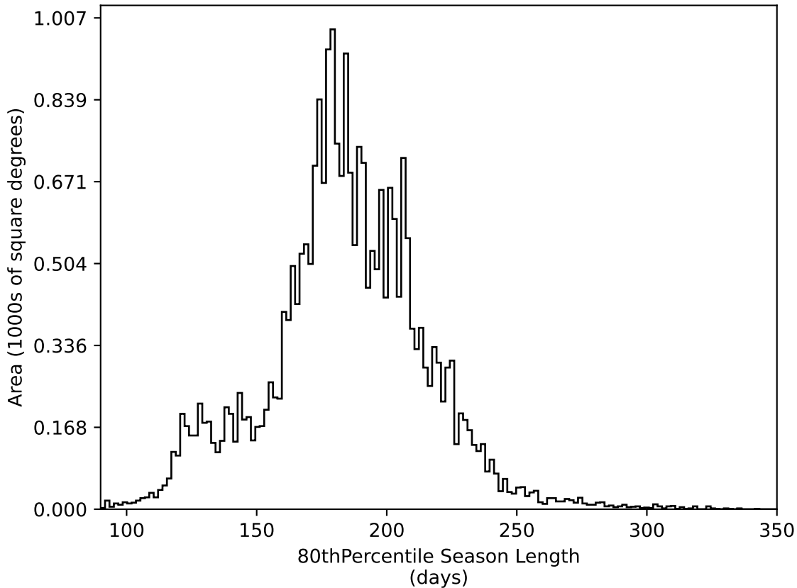
ddf_loaded_fl15_v3.4_10yrs All sky all bands: 80thPercentile Season Length
