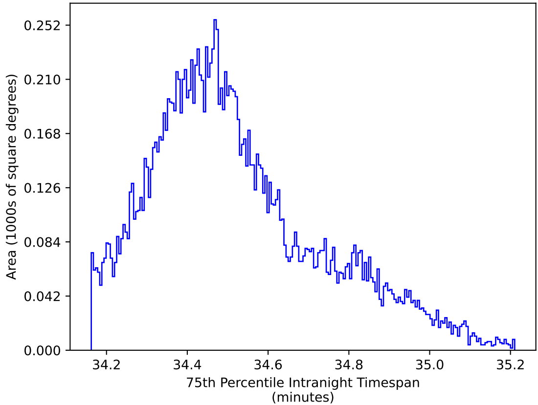
ddf_loaded_fl15_v3.4_10yrs WFD zy bands: 75th Percentile Intranight Timespan
