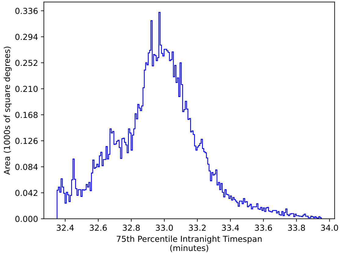
ddf_loaded_fl15_v3.4_10yrs WFD y band: 75th Percentile Intranight Timespan
