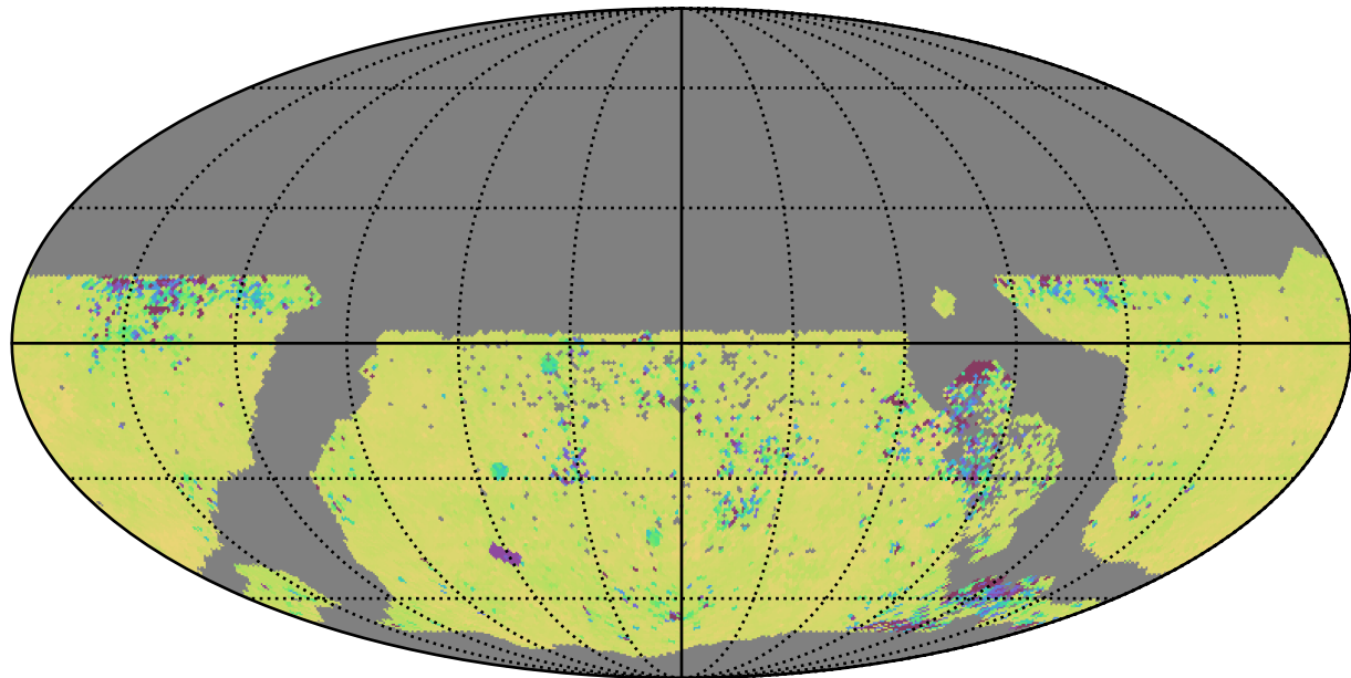
ddf_loaded_fl15_v3.4_10yrs WFD ug bands: 75th Percentile Intranight Timespan
