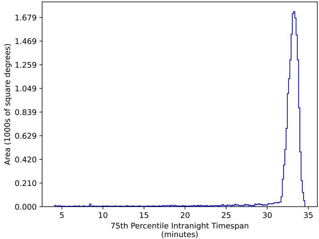
ddf_loaded_fl15_v3.4_10yrs WFD ug bands: 75th Percentile Intranight Timespan
