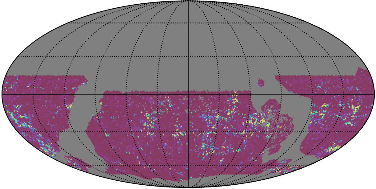
ddf_loaded_fl15_v3.4_10yrs WFD u band: 75th Percentile Intranight Timespan
