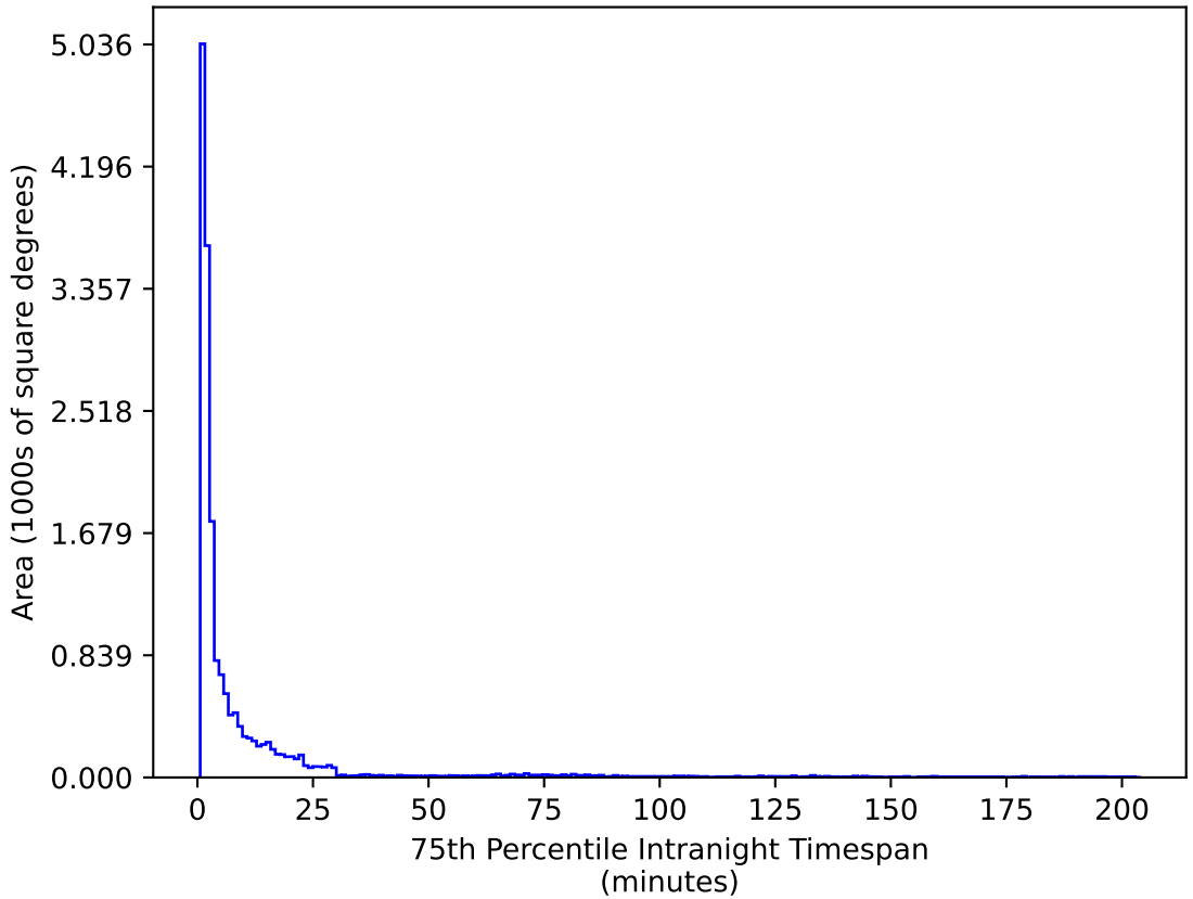
ddf_loaded_fl15_v3.4_10yrs WFD u band: 75th Percentile Intranight Timespan
