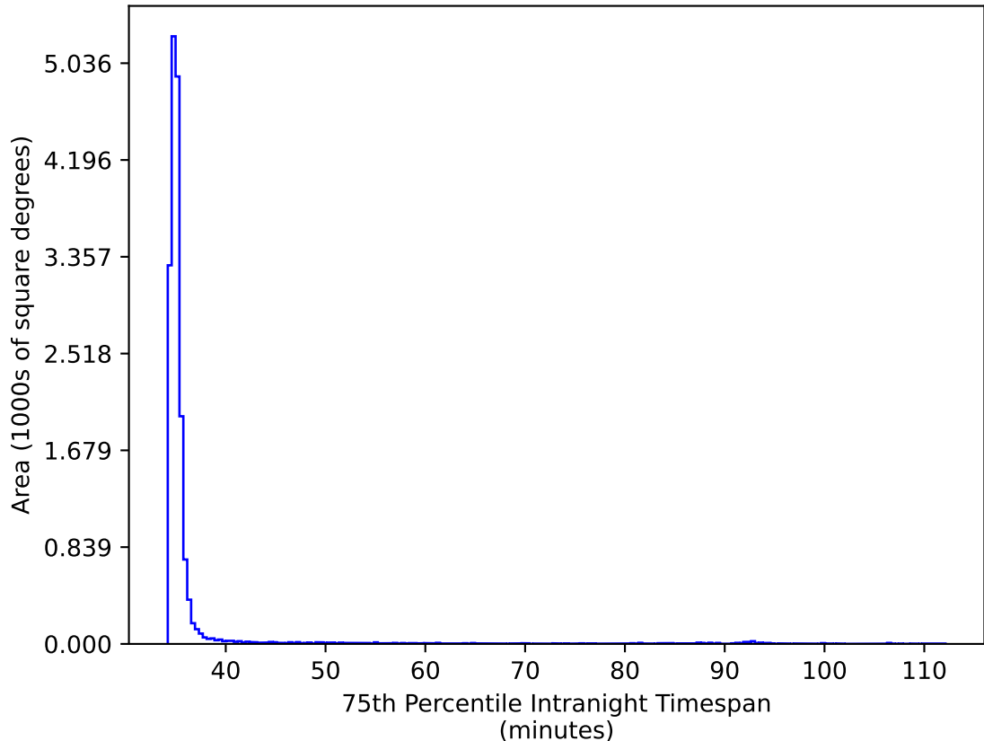
ddf_loaded_fl15_v3.4_10yrs WFD ri bands: 75th Percentile Intranight Timespan
