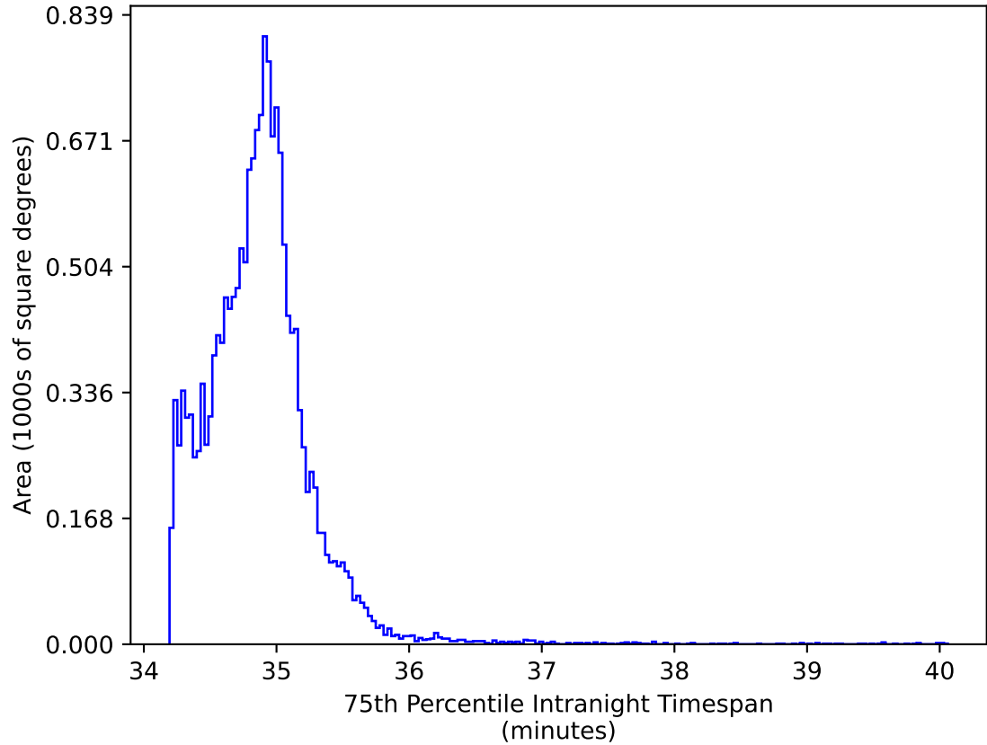
ddf_loaded_fl15_v3.4_10yrs WFD iz bands: 75th Percentile Intranight Timespan
