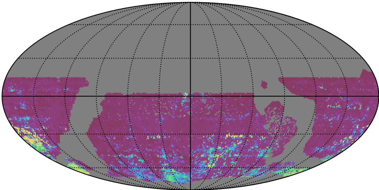
ddf_loaded_fl15_v3.4_10yrs WFD i band: 75th Percentile Intranight Timespan
