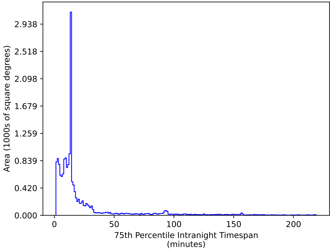
ddf_loaded_fl15_v3.4_10yrs WFD i band: 75th Percentile Intranight Timespan
