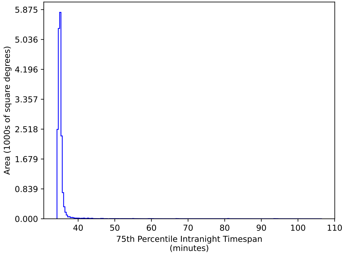
ddf_loaded_fl15_v3.4_10yrs WFD gr bands: 75th Percentile Intranight Timespan
