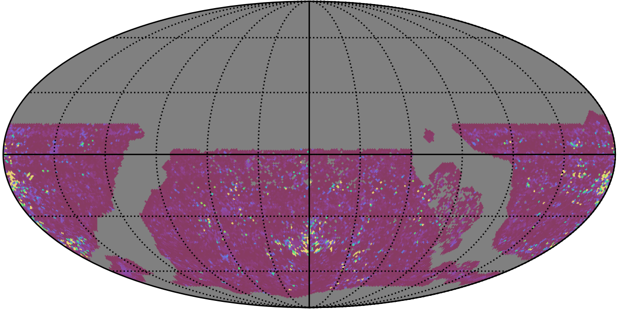
ddf_loaded_fl15_v3.4_10yrs WFD g band: 75th Percentile Intranight Timespan
