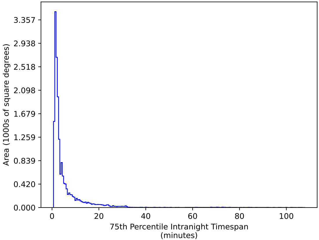
ddf_loaded_fl15_v3.4_10yrs WFD g band: 75th Percentile Intranight Timespan
