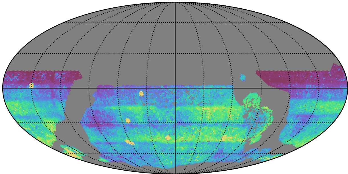
ddf_loaded_fl15_v3.4_10yrs WFD all bands: 75th Percentile Intranight Timespan
