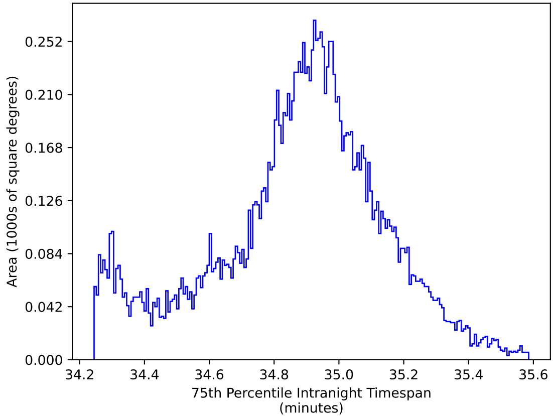
ddf_loaded_fl15_v3.4_10yrs WFD all bands: 75th Percentile Intranight Timespan
