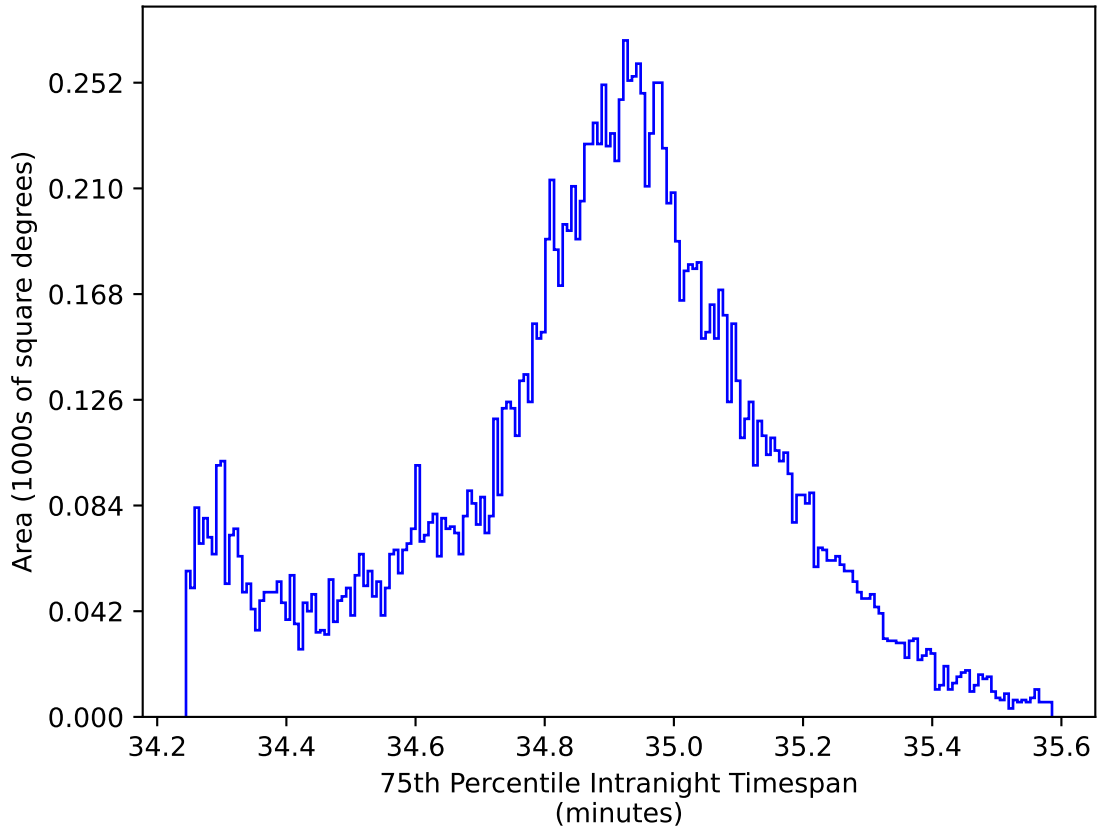
ddf_loaded_fl15_v3.4_10yrs WFD: 75th Percentile Intranight Timespan
