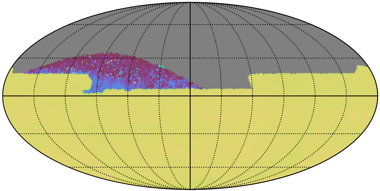
ddf_loaded_fl15_v3.4_10yrs All sky zy bands: 75th Percentile Intranight Timespan
