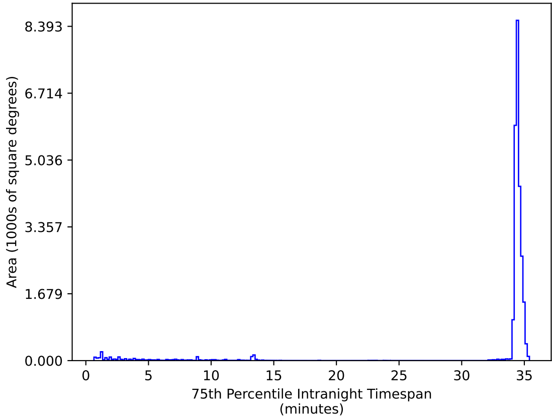
ddf_loaded_fl15_v3.4_10yrs All sky zy bands: 75th Percentile Intranight Timespan
