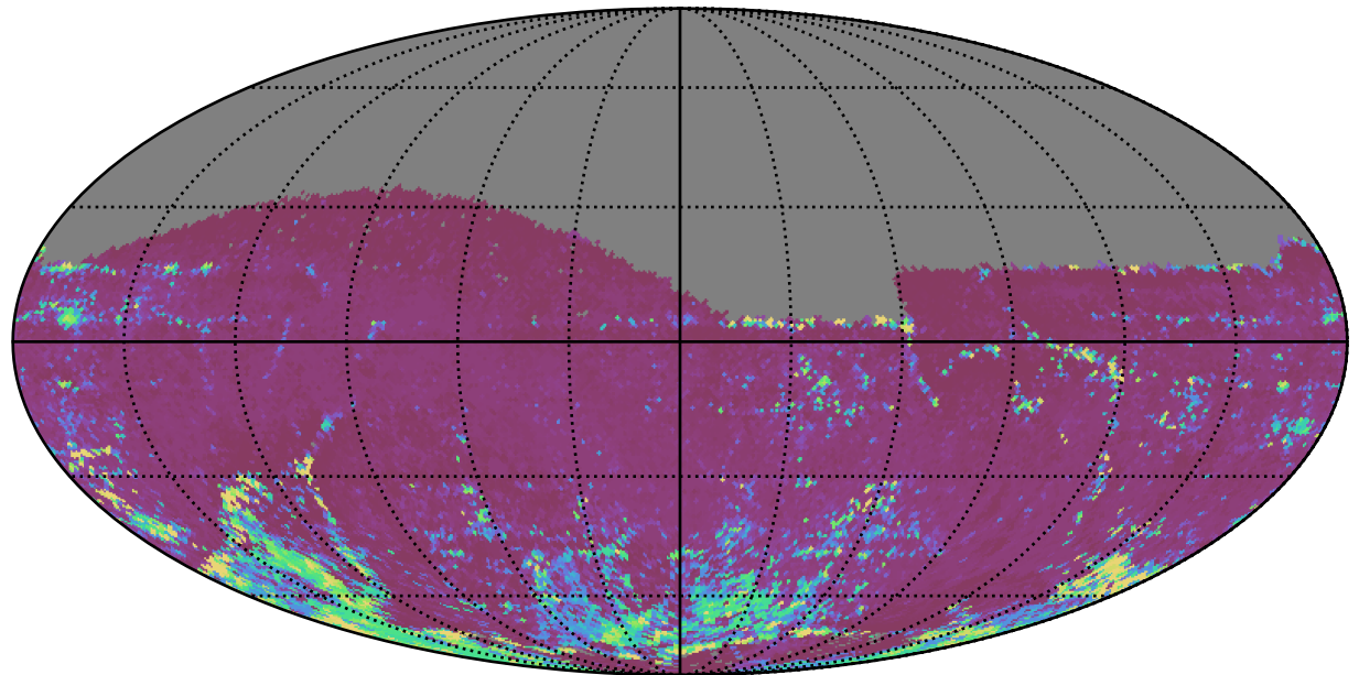
ddf_loaded_fl15_v3.4_10yrs All sky z band: 75th Percentile Intranight Timespan
