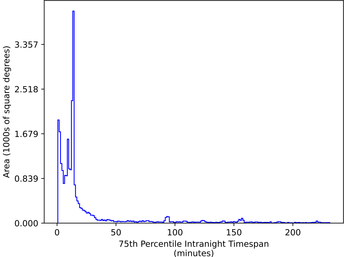
ddf_loaded_fl15_v3.4_10yrs All sky z band: 75th Percentile Intranight Timespan
