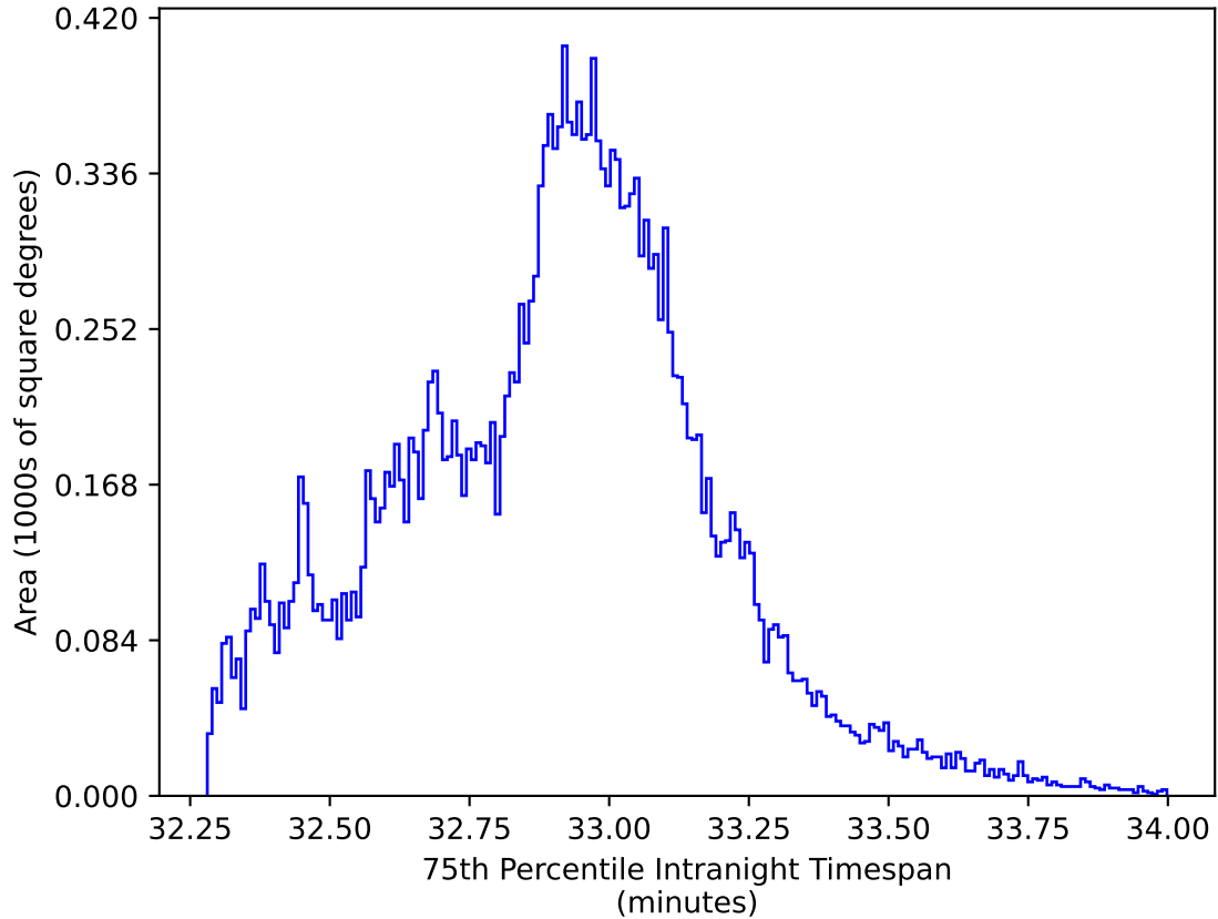
ddf_loaded_fl15_v3.4_10yrs All sky y band: 75th Percentile Intranight Timespan
