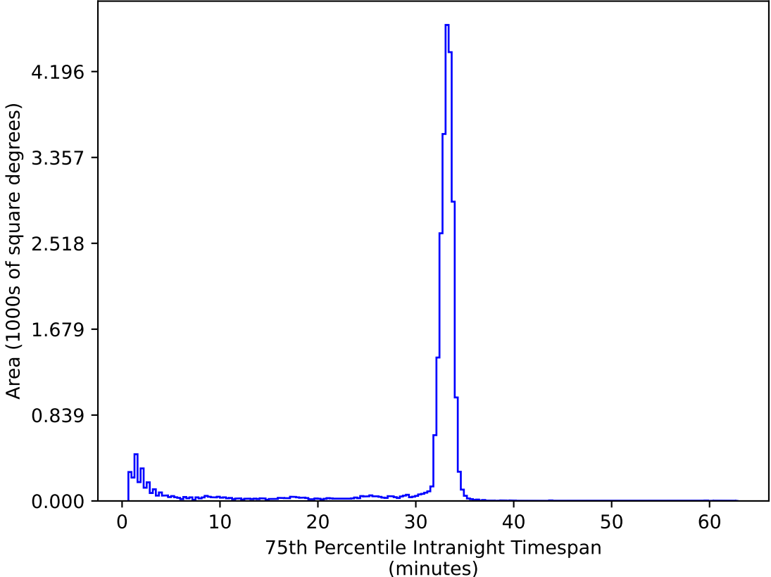
ddf_loaded_fl15_v3.4_10yrs All sky ug bands: 75th Percentile Intranight Timespan
