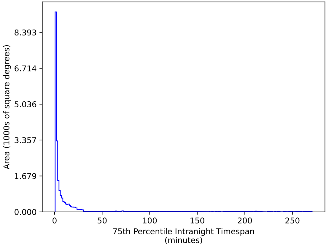
ddf_loaded_fl15_v3.4_10yrs All sky u band: 75th Percentile Intranight Timespan
