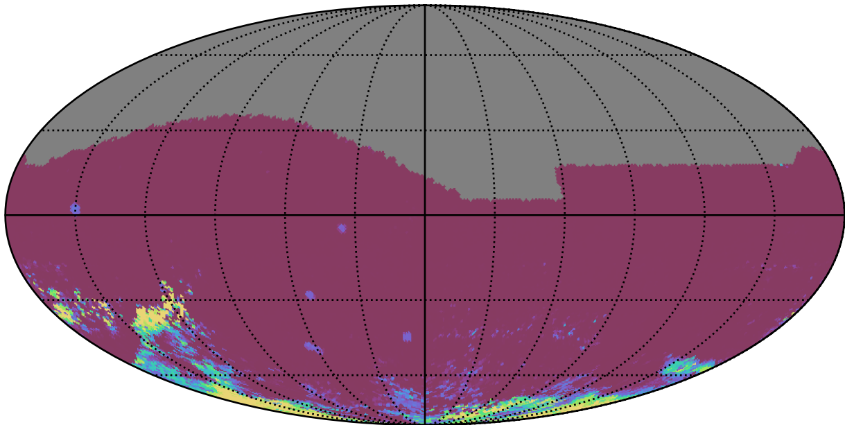
ddf_loaded_fl15_v3.4_10yrs All sky ri bands: 75th Percentile Intranight Timespan
