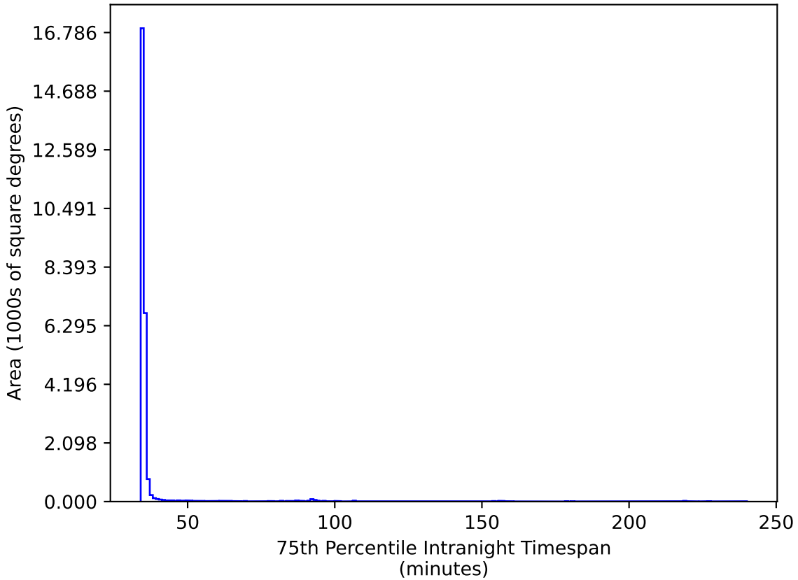
ddf_loaded_fl15_v3.4_10yrs All sky ri bands: 75th Percentile Intranight Timespan
