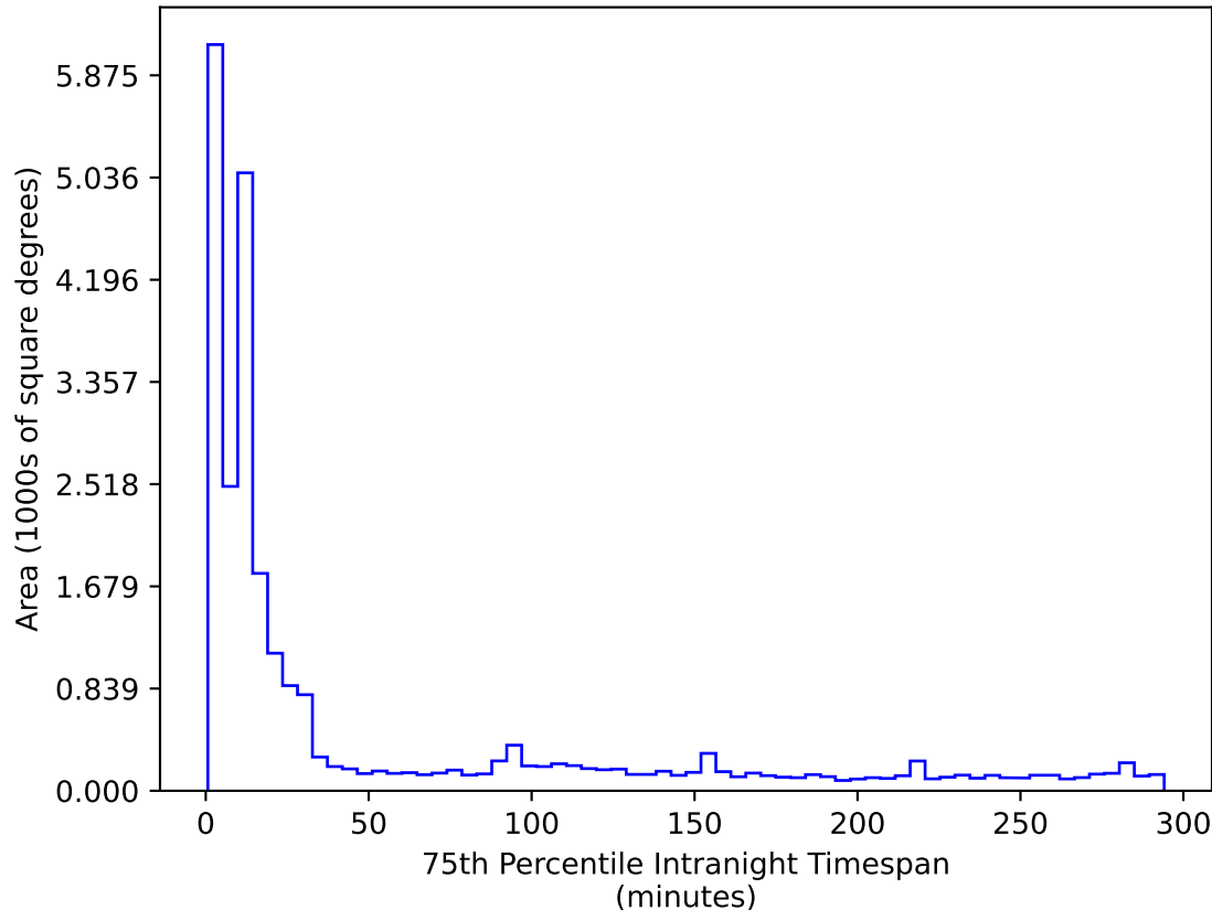
ddf_loaded_fl15_v3.4_10yrs All sky r band: 75th Percentile Intranight Timespan
