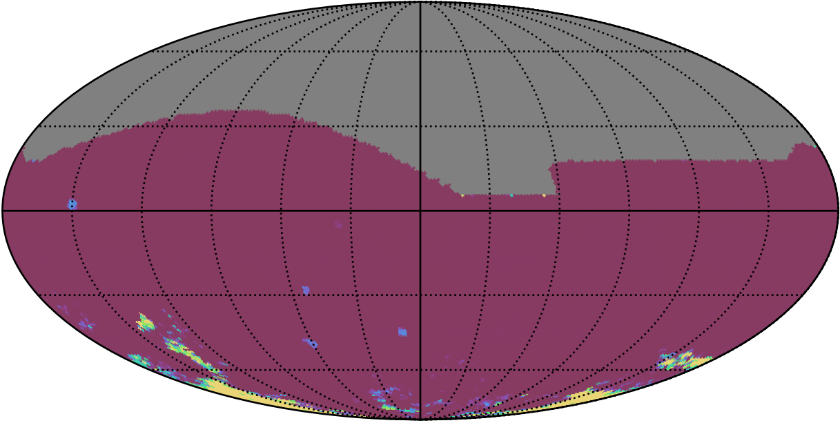
ddf_loaded_fl15_v3.4_10yrs All sky iz bands: 75th Percentile Intranight Timespan
