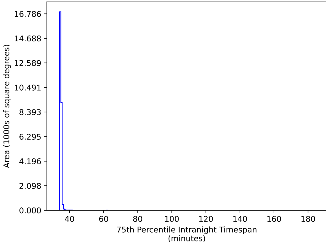
ddf_loaded_fl15_v3.4_10yrs All sky iz bands: 75th Percentile Intranight Timespan
