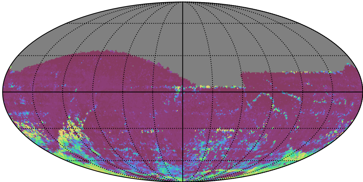
ddf_loaded_fl15_v3.4_10yrs All sky i band: 75th Percentile Intranight Timespan
