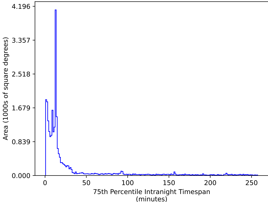
ddf_loaded_fl15_v3.4_10yrs All sky i band: 75th Percentile Intranight Timespan
