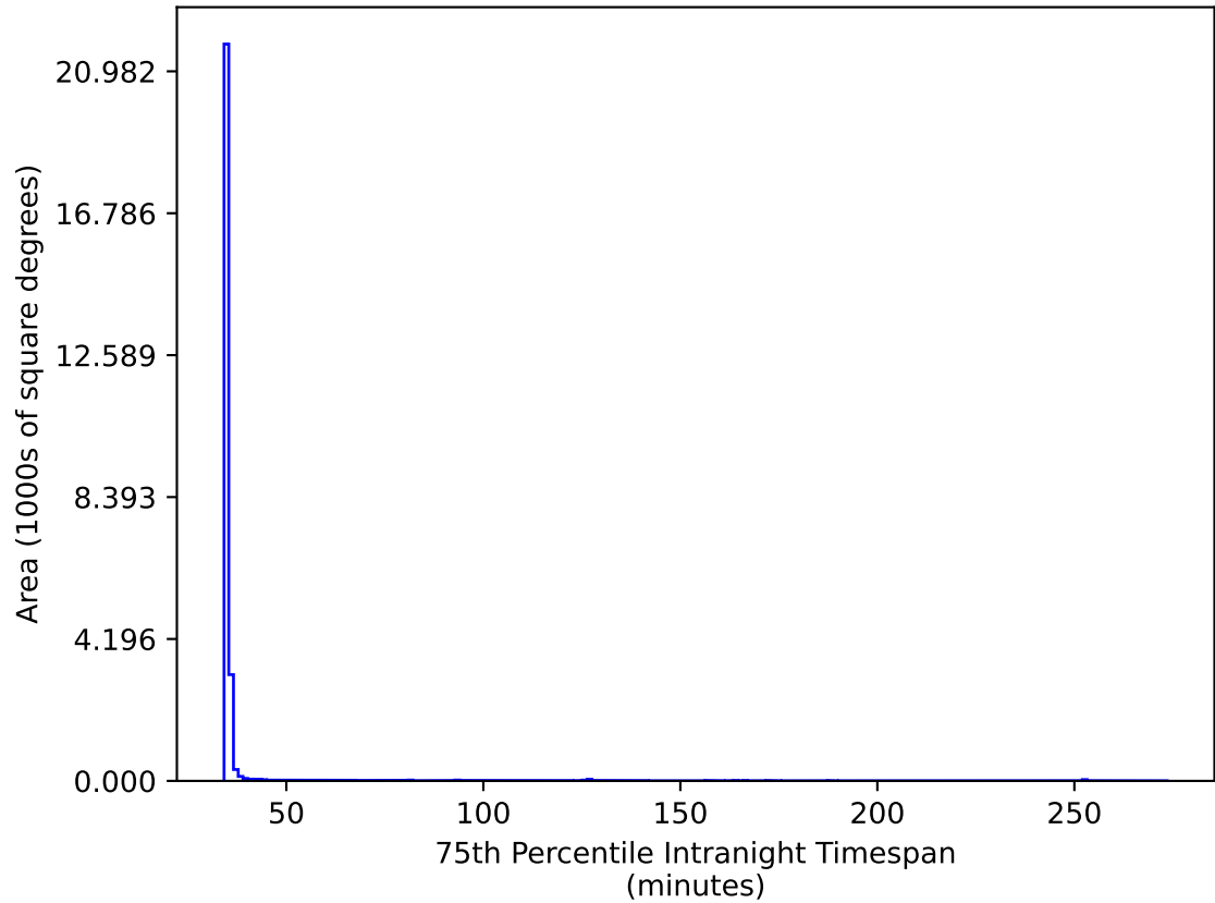
ddf_loaded_fl15_v3.4_10yrs All sky gr bands: 75th Percentile Intranight Timespan
