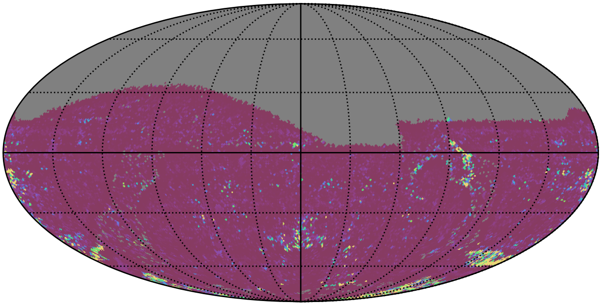
ddf_loaded_fl15_v3.4_10yrs All sky g band: 75th Percentile Intranight Timespan
